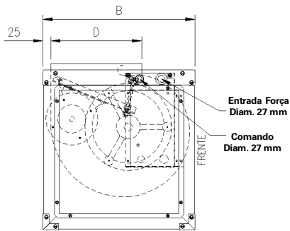
Fig. 11a - Descarga Vertical
